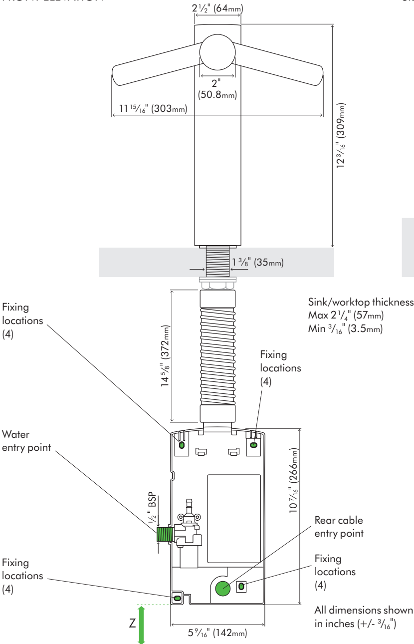
FRONT ELEVATION
