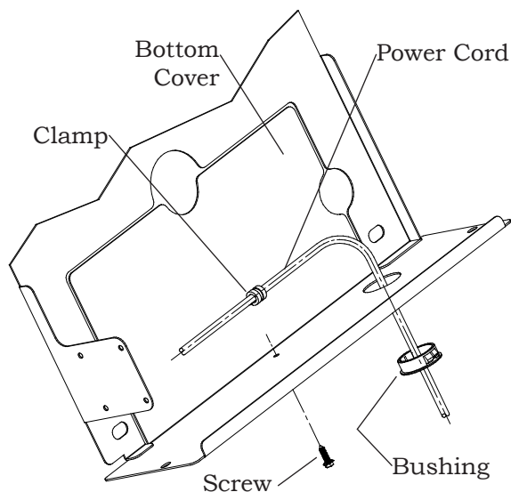
220V Power Cord Detail FIG. 5
