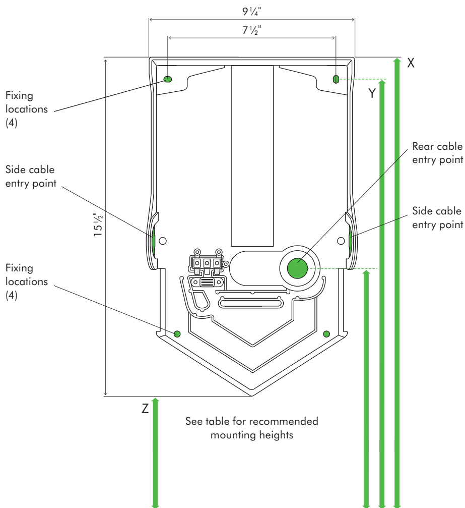
REAR ELEVATION
