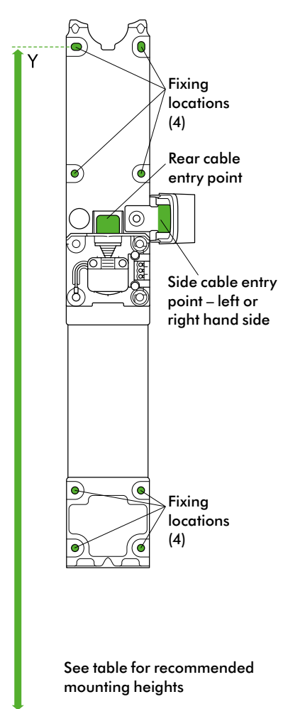
Back plate
